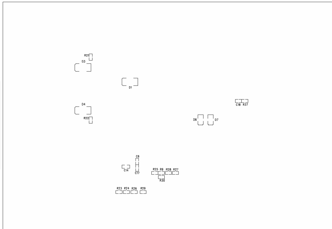
Figure 14. Bottom Silkscreen
