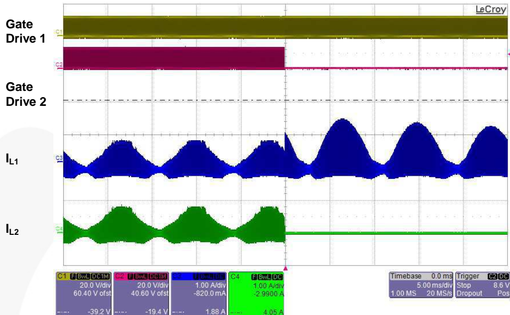
Figure 31. Phase-Shedding Operation
