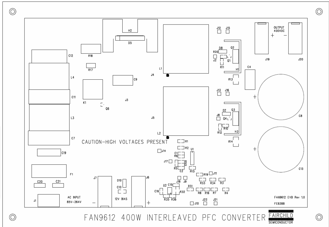
Figure 13. Top Silkscreen
