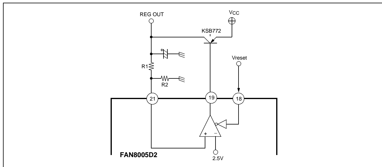
Figure 1. Regulator circuit
