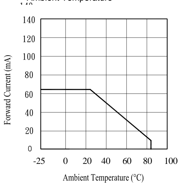
Fig.1 Forward Current vs. Ambient Temperature
