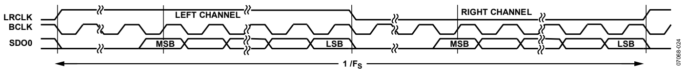
Figure 28. Right-Justified Mode
