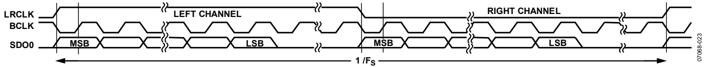
Figure 27. Left-Justified Mode
