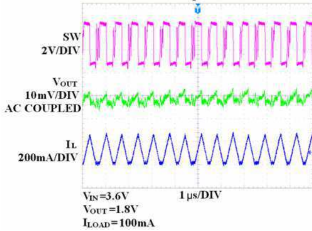
Discontinuous Operation
