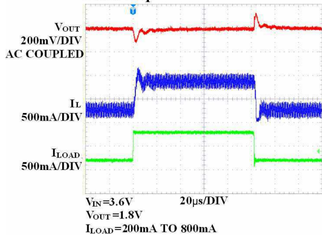
Load Step
