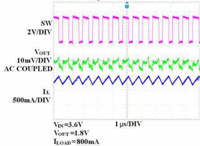
Normal Operation
