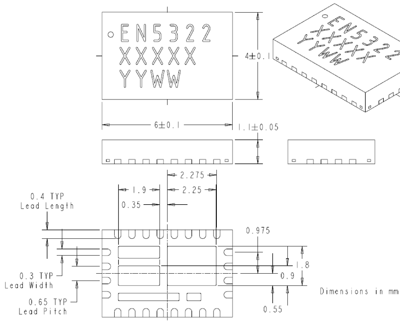
Figure 7. EN5322QI Package Dimensions
