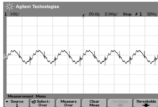
Fig. 19 Typical output ripple voltage AVQ100B -48S3V3, room temperature, lo = lo,max
