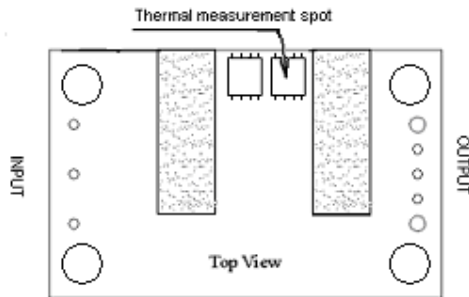
Fig.62 Temperature measurement location
