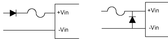
Fig. 59 Reverse polarity protection circuit
