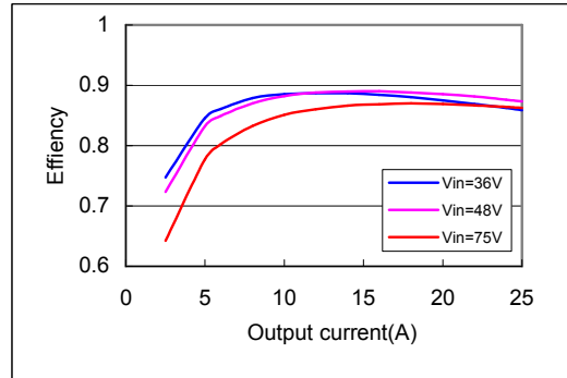
Fig. 2 Typical efficiency of AGQ100-48S1V5
