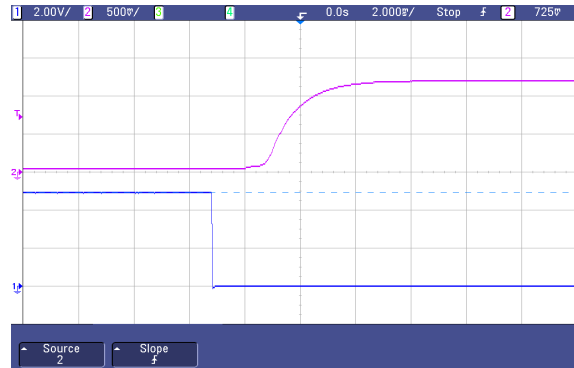
Fig.22 Typical start-up from CNT on of AGQ100-48S1V2
