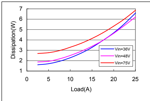
Fig. 13 Typical power dissipation curve of AGQ100-48S1V8
