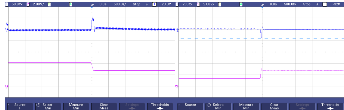
Fig.31 Typical transient response to step decrease in load from 50% to 25%, room temperature, 48Vdc input ( \Delta I_o/\Delta t = 0.1A/1\mu s ) of AGQ100-48S1V2
