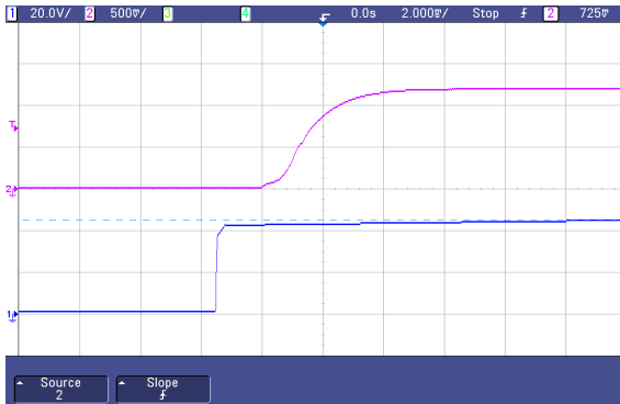
Fig.21 Typical start-up from power on of AGQ100-48S1V2
