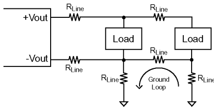
Fig. 57 Ground loops
