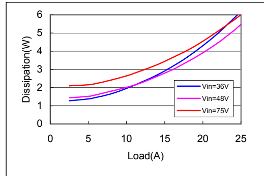
Fig. 12 Typical power dissipation curve of AGQ100-48S1V5
