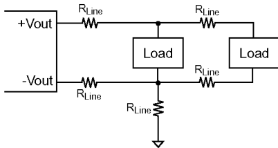
Fig. 58 Single point ground
