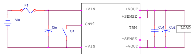
Fig. 60 Typical application
