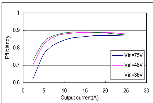
Fig. 3 Typical efficiency of AGQ100-48S1V8
