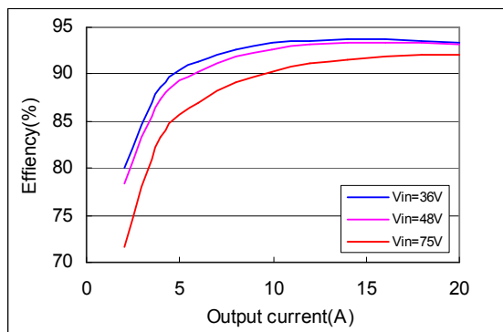
Fig. 5 Typical efficiency of AVQ100B-48S05
