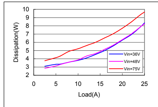
Fig. 14 Typical power dissipation curve of AVQ100B-48S3V3
