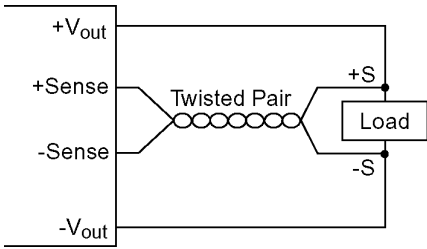
Fig. 52 Sense connections
