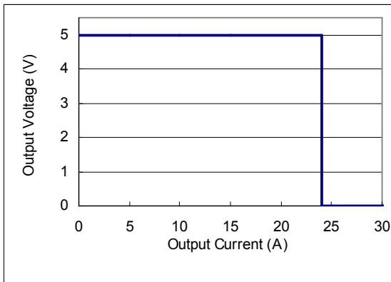
Fig. 10 Typical over-current of AVQ100B-48S05
