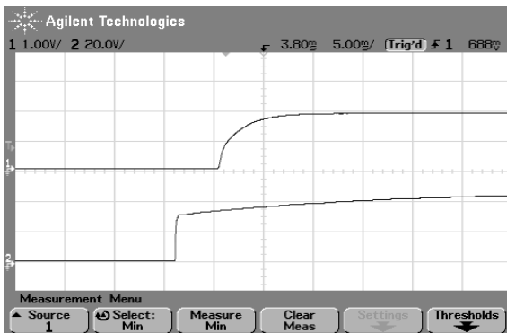
Fig.25 Typical start-up from power on of AGQ100-48S1V8
