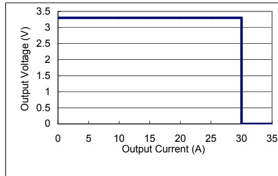
Fig. 9 Typical over-current of AVQ100B-48S3V3
