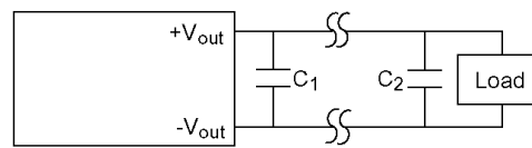
Fig. 56 Output ripple filter for a distant load
