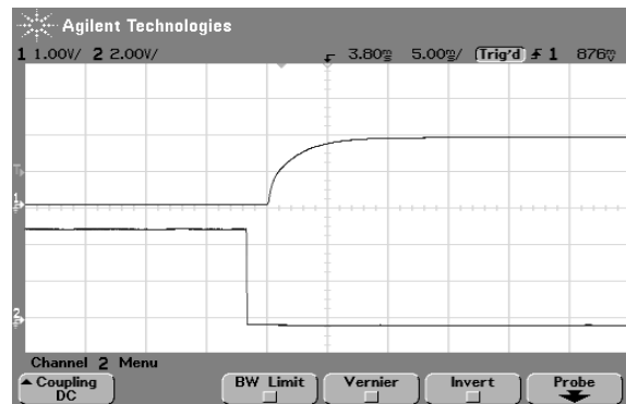
Fig.26 Typical start-up from CNT on of AGQ100-48S1V8
