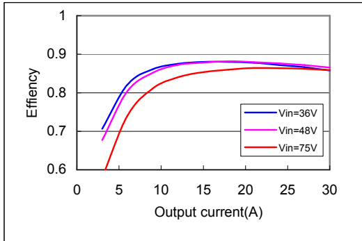
Fig. 1 Typical efficiency of AGQ100-48S1V2
