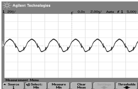
Fig. 18 Typical output ripple voltage AGQ100 -48S1V8, room temperature, lo = lo,max
