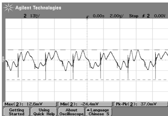
Fig. 20 Typical output ripple voltage AVQ100B -48S05, room temperature, lo = lo,max
