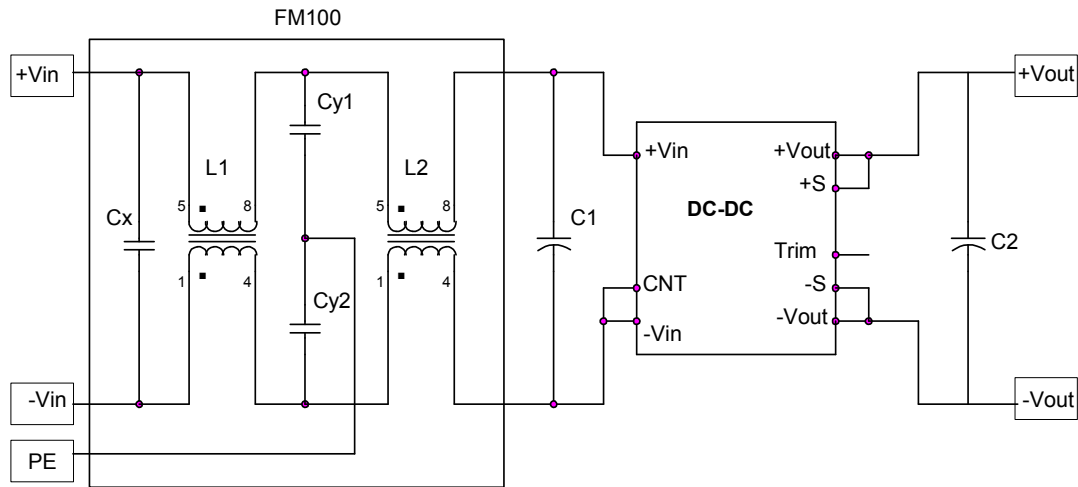
Figure 61 EMI reduction filter
