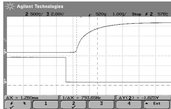
Fig.24 Typical start-up from CNT on of AGQ100-48S1V5
