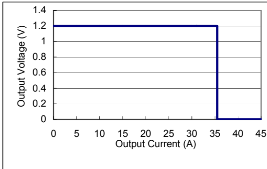
Fig. 6 Typical over-current of AGQ100-48S1V2
