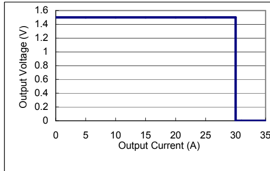
Fig. 7 Typical over-current of AGQ100-48S1V5
