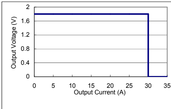
Fig. 8 Typical over-current of AGQ100-48S1V8
