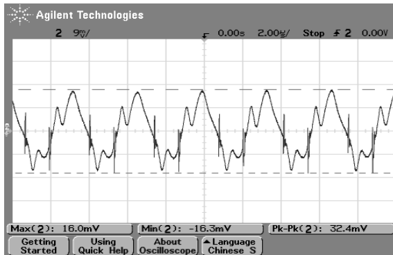
Fig. 16 Typical output ripple voltage AGQ100 -48S1V2, room temperature, lo = lo,max
