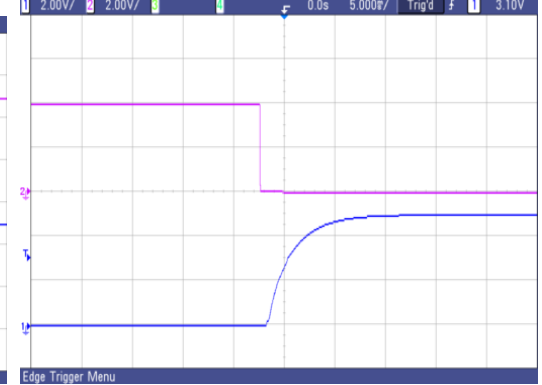
Fig.30 Typical start-up from CNT on of AVQ100B-48S05
