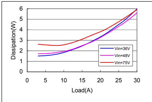
Fig. 11 Typical power dissipation curve of AGQ100-48S1V2
