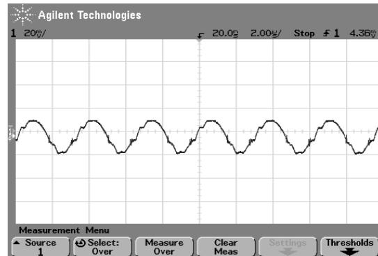
Fig. 17 Typical output ripple voltage AGQ100 -48S1V5, room temperature, lo = lo,max
