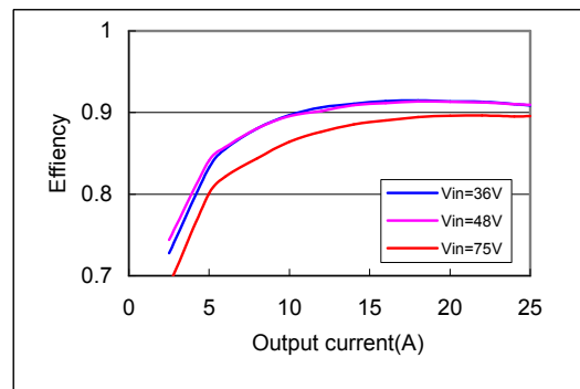
Fig. 4 Typical efficiency of AVQ100B-48S3V3
