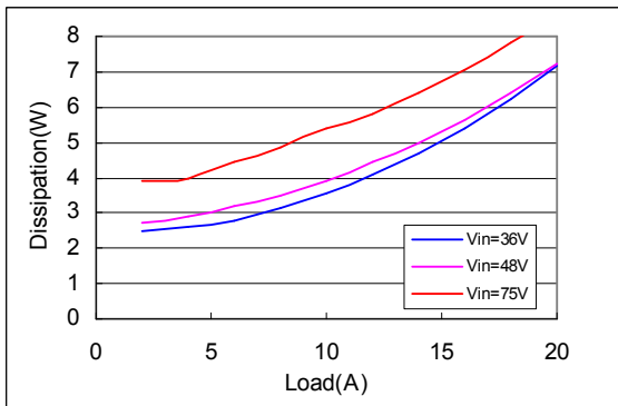
Fig. 15 Typical power dissipation curve of AVQ100B-48S05
