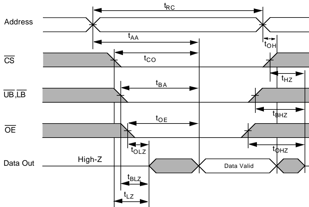
TIMING WAVEFORM OF READ CYCLE(2) ( \overline{WE} = V_{IH} )
