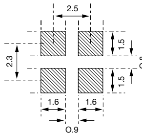
Figure 2) Land Pattern
