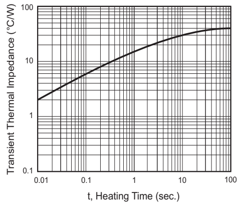
Figure 6. Typical Transient Thermal Impedance
