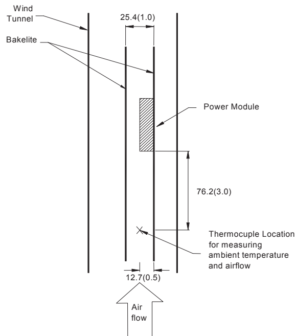
Note : Dimensions are in millimeters and (inches) Figure 6. Thermal Test Setup
