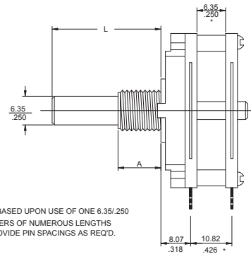
Typical Assembled Switch
