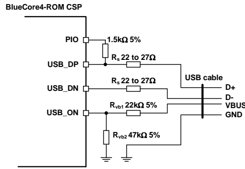
Figure 11.12: USB Connections for Self Powered Mode
