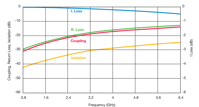
CP0402AxxxxFLTR
