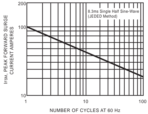
FIG. 6 - MAXIMUM NON-REPETITIVE FORWARD SURGE CURRENT UNI-DIRECTIONAL
