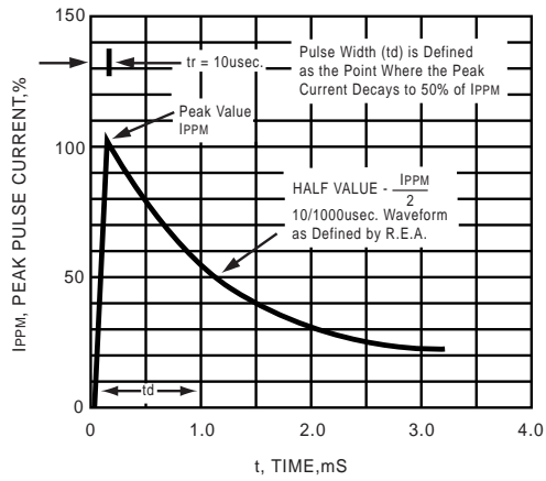
FIG. 3 - PULSE WAVEFORM
