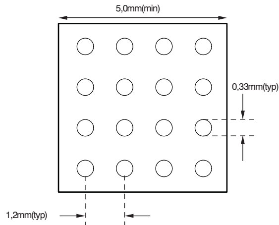
Figure 12. Recommended PCB Layout
