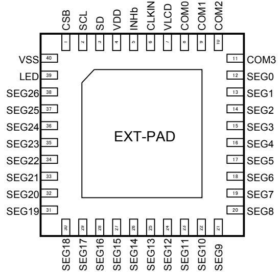
Fig.6 Pin Arrangement (BU97930MUV)
