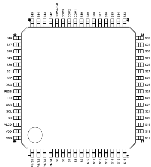
Fig.14 Pin Arrangement (BU97500KV)
