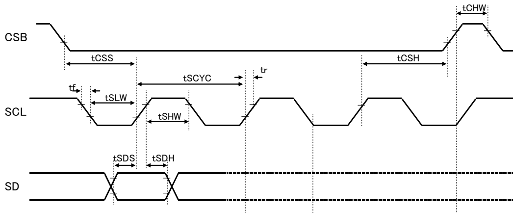
Fig.4 Serial interface Timing
