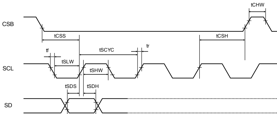
Fig.1 Serial Interface Timing
