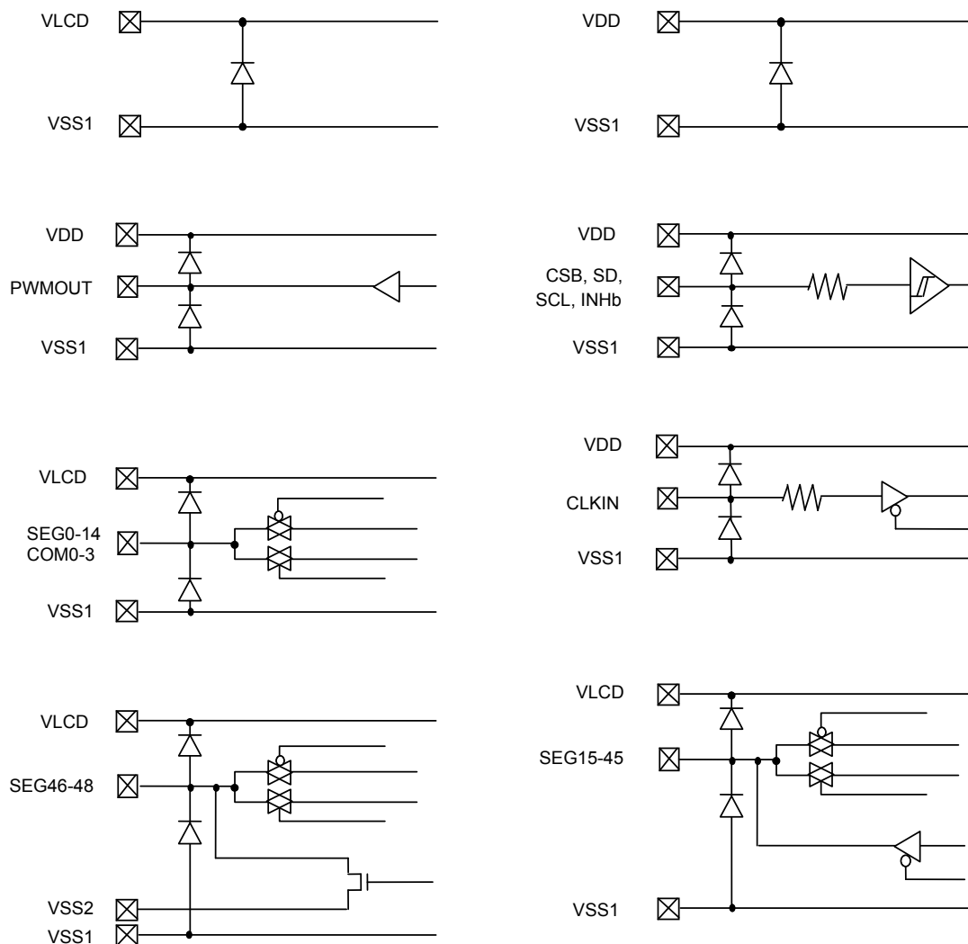
Fig.18 I/O equivalent circuit
