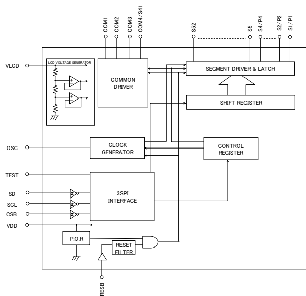
Fig.13 Block Diagram (BU97500KV)
