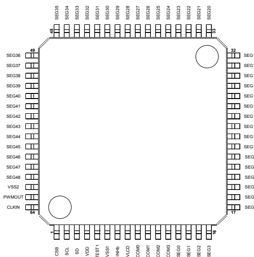
Fig.10 Pin Arrangement (BU9798KV)
