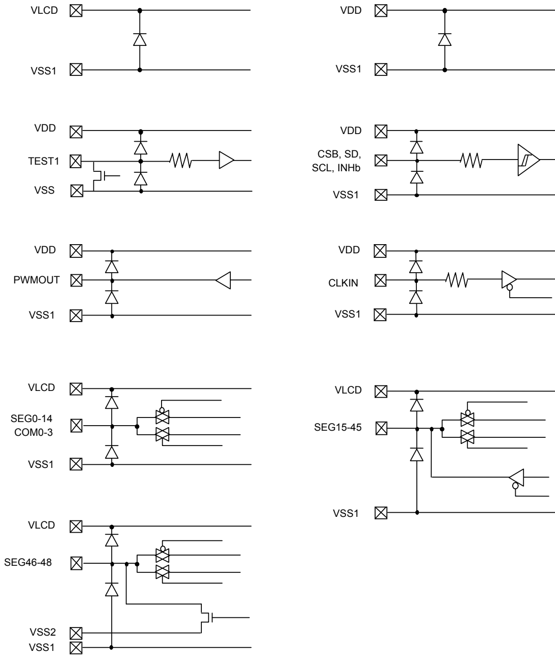
Fig.17 I/O equivalent circuit
