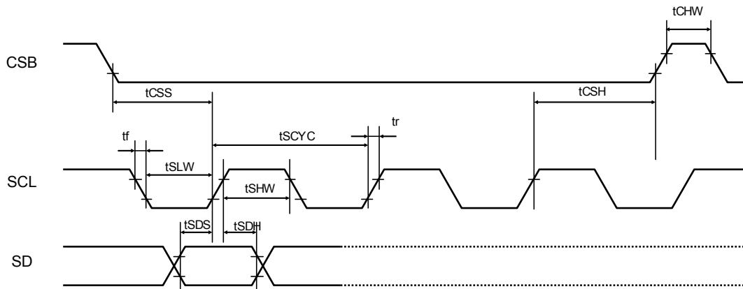
Fig.3 Serial Interface Timing
