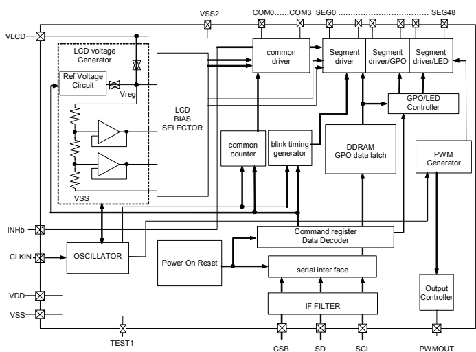
Fig.9 Block Diagram (BU9798KV)
