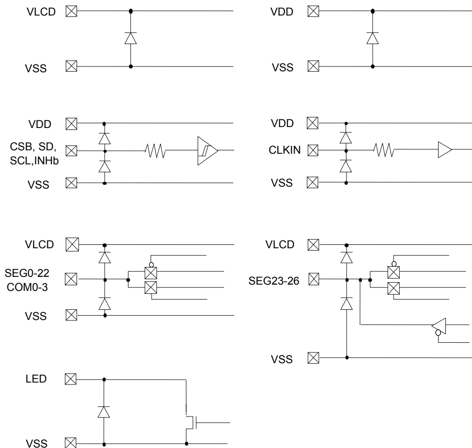
Fig.15 I/O equivalent circuit
