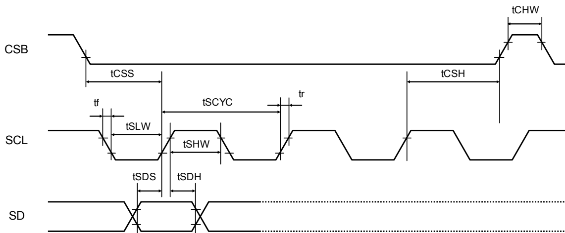
Fig.2 Serial Interface Timing
