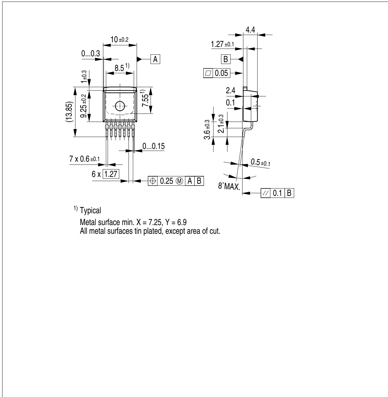
Figure 20 PG-TO220-7-4
