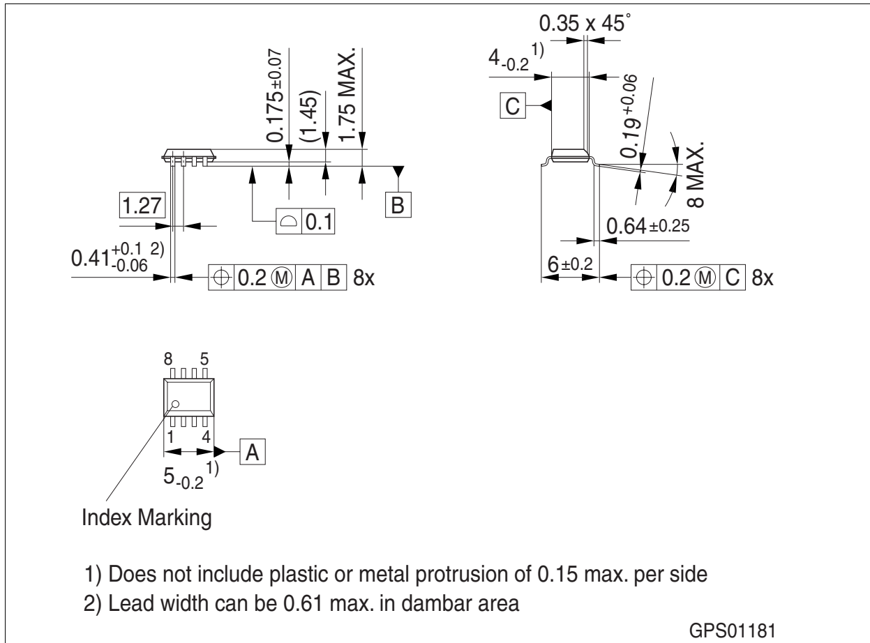
Figure 1 PG-DSO8-25 (Plastic Green Dual Small Outline Package)
