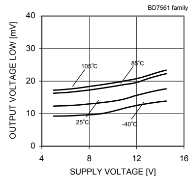
Fig. 7 Output Voltage Low – Supply Voltage ( R_L=10[k\Omega] )
