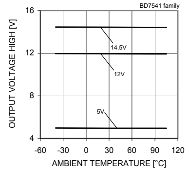
Fig. 52 Output Voltage High - Ambient Temperature (RL=10[kΩ])
