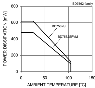
Fig. 25 Derating Curve
