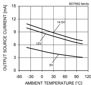
Fig. 33 Output Source Current – Ambient Temperature
