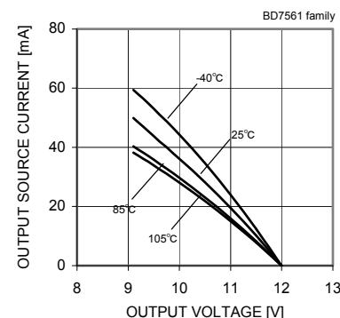
Fig. 9 Output Source Current – Output Voltage ( V_{DD}=12[V] )
