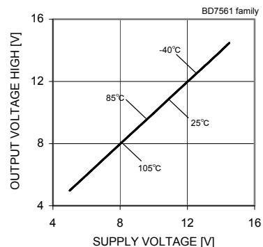
Fig. 5 Output Voltage High – Supply Voltage ( R_L=10[k\Omega] )
