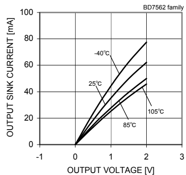
Fig. 34 Output Sink Current – Output Voltage (VDD=12[V])
