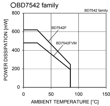
Fig. 70 Derating Curve
