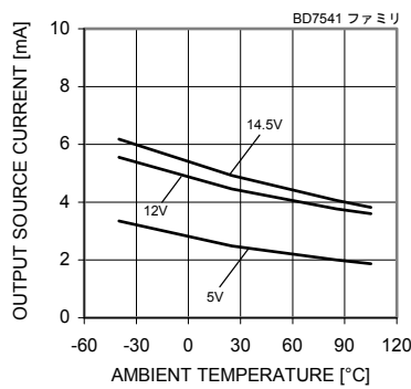
Fig. 56 Output Source Current - Ambient Temperature
