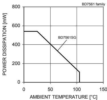
Fig. 2 Derating Curve
