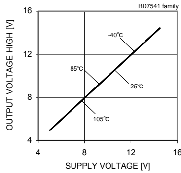
Fig. 51 Output Voltage High - Supply Voltage (RL=10[kΩ])
