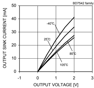
Fig. 80 Output Sink Current – Output Voltage ( V_{DD}=12[V] )
