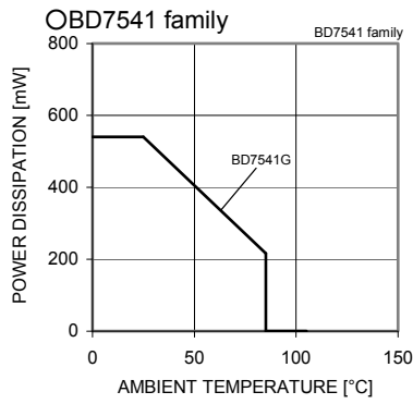
Fig. 47 Derating Curve
