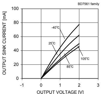
Fig. 11 Output Sink Current – Output Voltage ( V_{DD}=12[V] )
