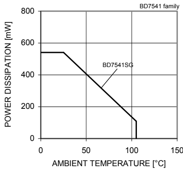
Fig. 48 Derating Curve
