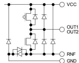
Fig.47 OUT1 / OUT2 (HSOP25/HSOPM28)
