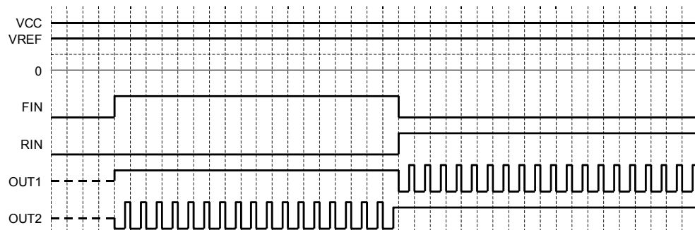
Fig.42 VREF control operation (timing chart)
