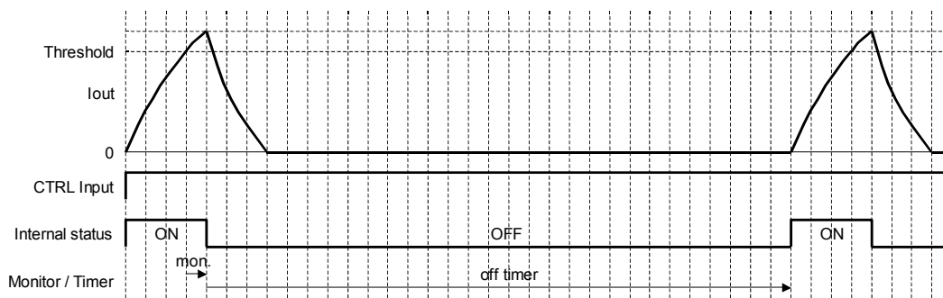
Fig.43 Over current protection (timing chart)
