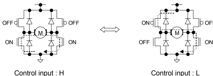
Fig.40 PWM control mode B operation (output stage)
