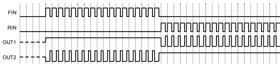
Fig.39 PWM control mode A operation (timing chart)
