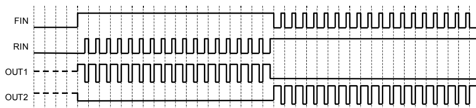
Fig.41 PWM control mode B operation (timing chart)
