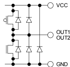
Fig.46 OUT1 / OUT2 (SOP8/HRP7)
