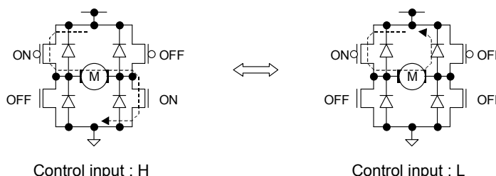
Fig.38 PWM control mode A operation (output stage)
