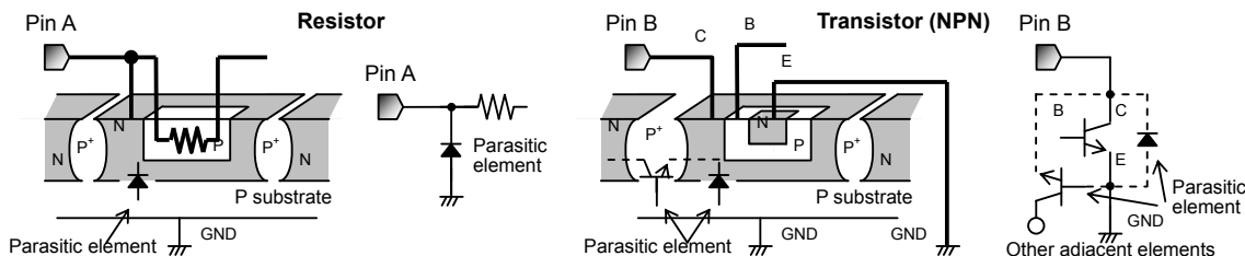
Appendix: Example of monolithic IC structure
