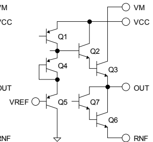
Fig.37 BA6920FP-Y
