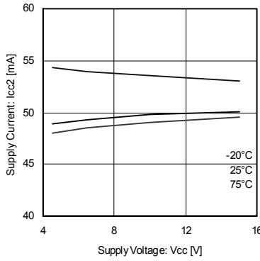
Fig.4 Supply current 2 (brake) (BA6287F)
