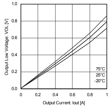
Fig. 18 Output low voltage (BA6285FS)
