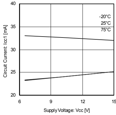
Fig.5 Supply current 1 (forward) (BA6285FS)
