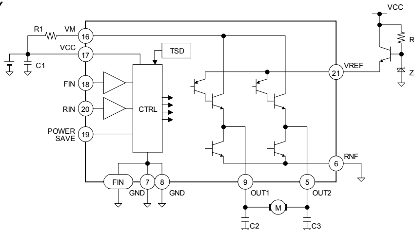
Fig.31 BA6285AFP-Y
