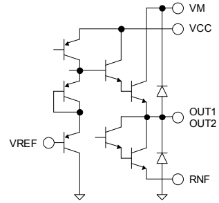
(BA6285FS, BA6285AFP-Y, BA6920FP-Y) Fig.39 POWER SAVE
