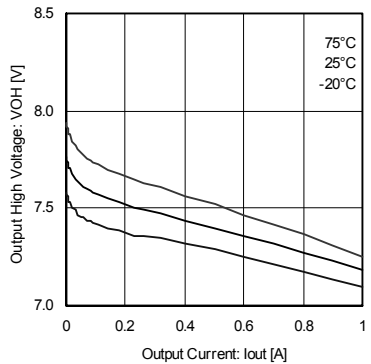
Fig.11 Output high voltage (BA6956AN)
