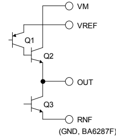
Fig.35 BA6287F, BA6285FS, BA6285AFP-Y
