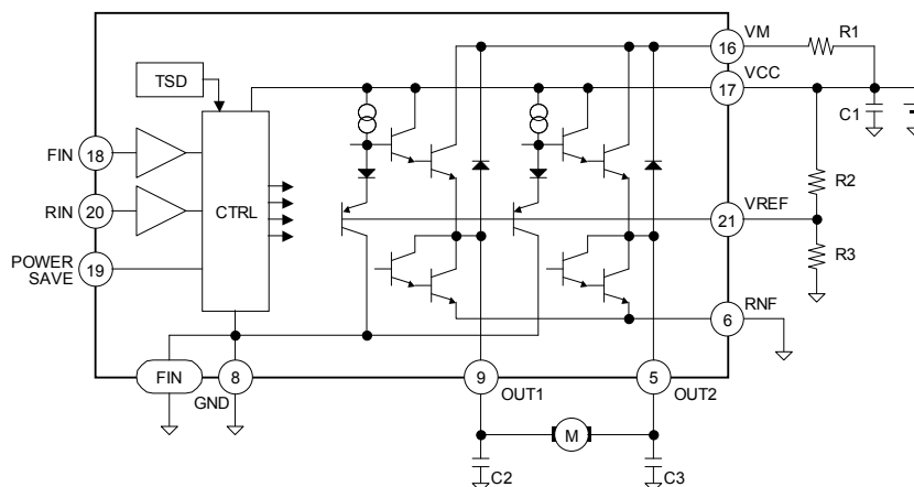
Fig.33 BA6920FP-Y
