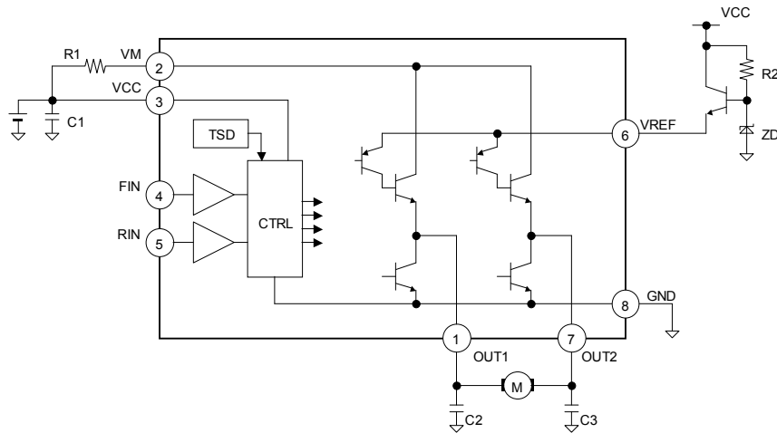
Fig.27 BA6287F
