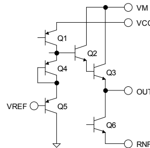
Fig.36 BA6956AN
