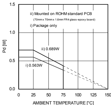
Fig. 22 Thermal derating curve (SOP8)
