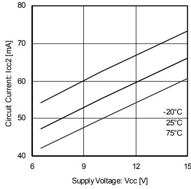
Fig.2 Supply current 2 (brake) (BA6956AN)
