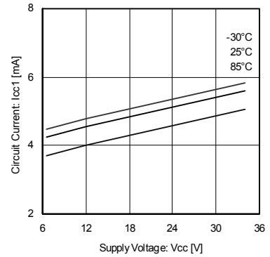
Fig.9 Supply current 1 (forward) (BA6920FP-Y)
