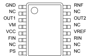
Fig.30 BA6285FS (SSOP-A16)
