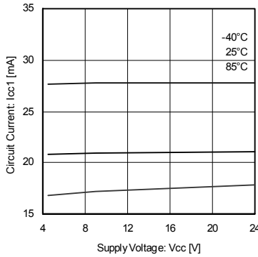
Fig.7 Supply current 1 (forward) (BA6285AFP-Y)
