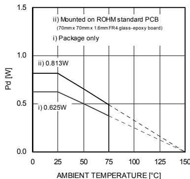
Fig. 23 Thermal derating curve (SSOP-A16)
