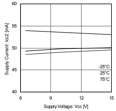
Fig.6 Supply current 2 (brake) (BA6285FS)
