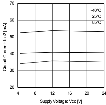
Fig.8 Supply current 2 (brake) (BA6285AFP-Y)
