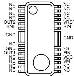
Fig.34 BA6920FP-Y (HSOP25)
