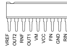
Fig.26 BA6956AN (SIP9)
