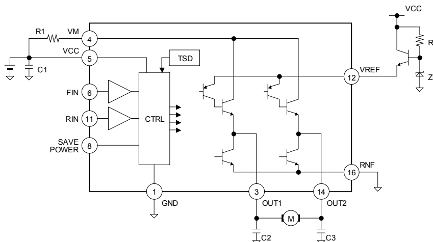
Fig.29 BA6285FS
