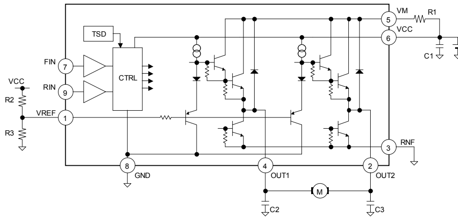
Fig.25 BA6956AN
