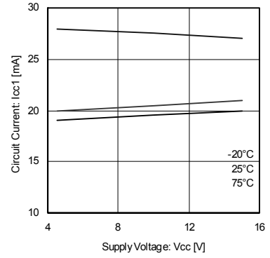
Fig.3 Supply current 1 (forward) (BA6287F)
