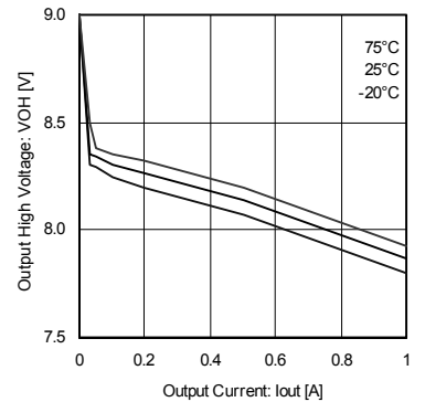
Fig.12 Output high voltage (BA6287F)
