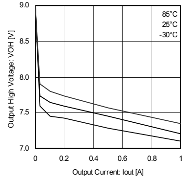
Fig. 15 Output high voltage (BA6920FP-Y)
