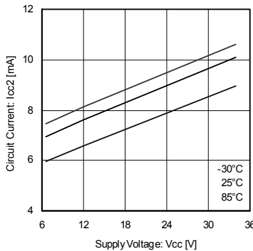
Fig.10 Supply current 2 (brake) (BA6920FP-Y)
