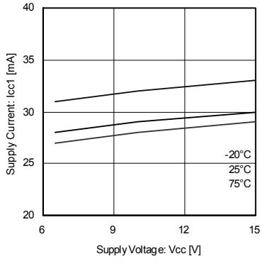
Fig.1 Supply current 1 (forward) (BA6956AN)
