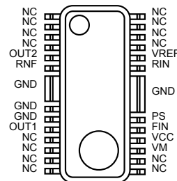
Fig.32 BA6285AFP-Y (HSOP25)
