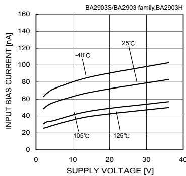
Fig. 50 Input Bias Current - Supply Voltage
