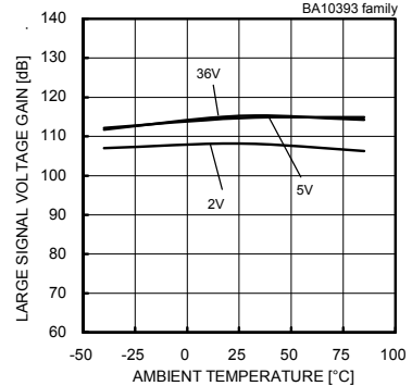
Fig. 15 Large Signal Voltage Gain – Ambient Temperature
