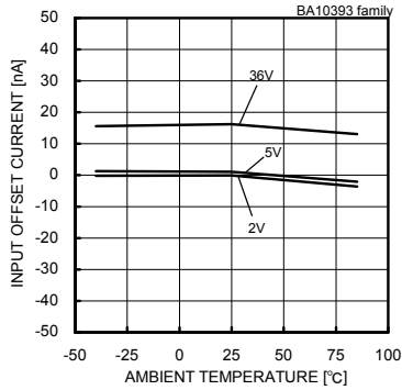
Fig. 13 Input Offset Current – Ambient Temperature
