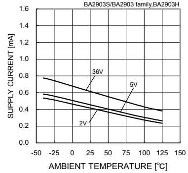
Fig. 43 Supply Current - Ambient Temperature
