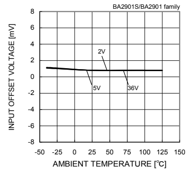
Fig. 72 Input Offset Voltage - Ambient Temperature
