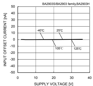
Fig. 52 Input Offset Current - Supply Voltage
