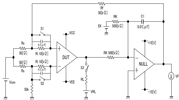
Fig.88 Measurement circuit1 (one channel only)
