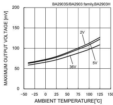
Fig. 45 Maximum Output Voltage - Ambient Temperature (IOL=4[mA])
