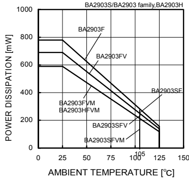
Fig. 41 Derating Curve
