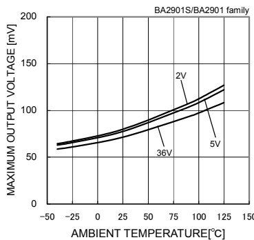
Fig. 68 Maximum Output Voltage - Ambient Temperature (IOL=4[mA])
