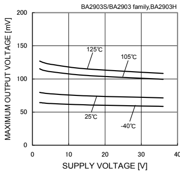
Fig. 44 Maximum Output Voltage - Supply Voltage (IOL=4[mA])
