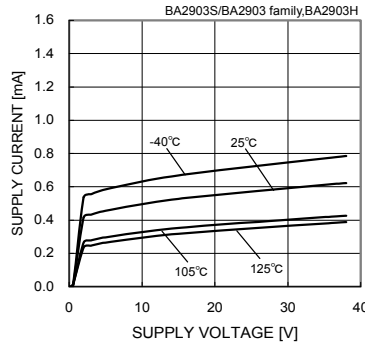
Fig. 42 Supply Current - Supply Voltage
