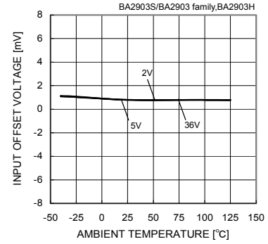
Fig. 49 Input Offset Voltage - Ambient Temperature
