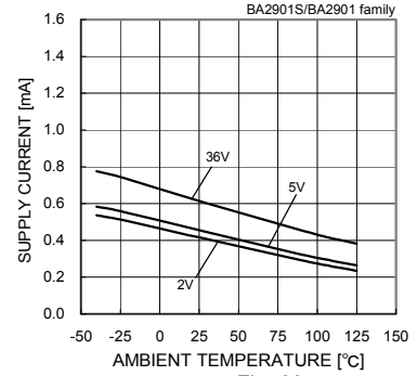
Fig. 66 Supply Current - Ambient Temperature
