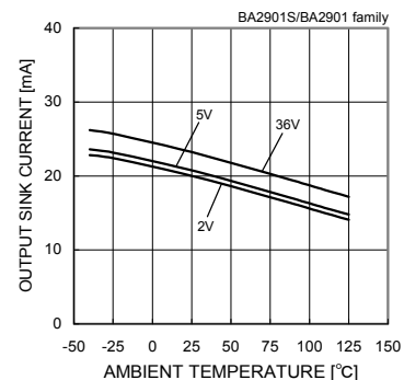
Fig. 70 Output Sink Current - Ambient Temperature (VOUT=1.5[V])
