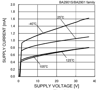
Fig. 65 Supply Current - Supply Voltage
