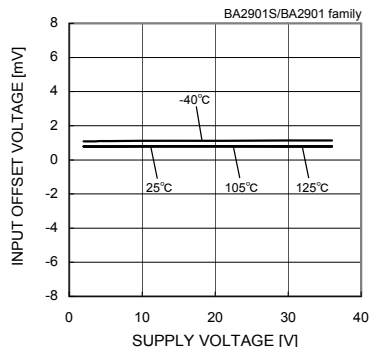
Fig. 71 Input Offset Voltage - Supply Voltage
