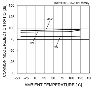
Fig. 80 Common Mode Rejection Ratio – Ambient Temperature
