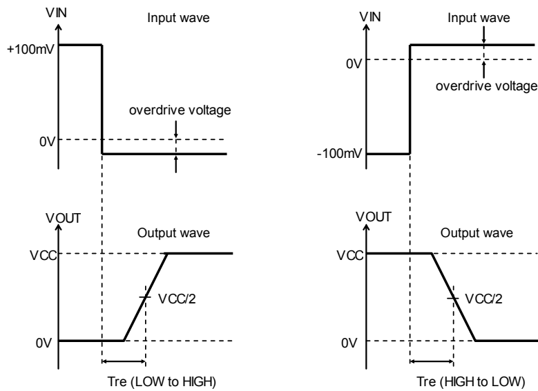
Fig.90 Response Time
