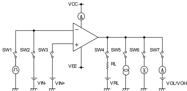
Fig.89 Measurement Circuit 2 (one channel only)
