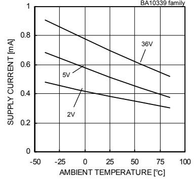
Fig. 23 Supply Current - Ambient Temperature
