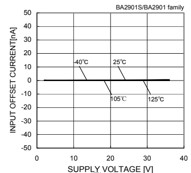
Fig. 75 Input Offset Current - Supply Voltage
