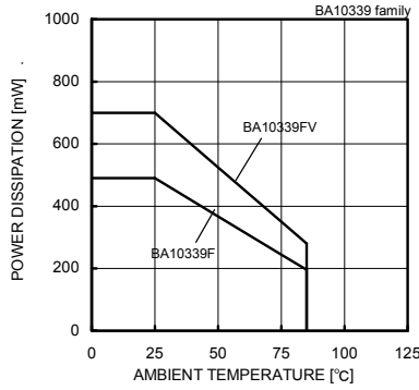
Fig. 21 Derating Curve
