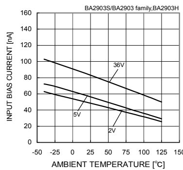
Fig. 51 Input Bias Current - Ambient Temperature
