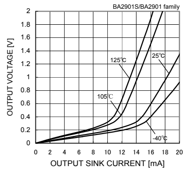
Fig. 69 Output Voltage - Output Sink Current (VCC=5[V])
