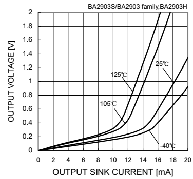
Fig. 46 Output Voltage - Output Sink Current (VCC=5[V])
