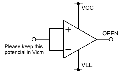
Fig.93 Disable circuit example
