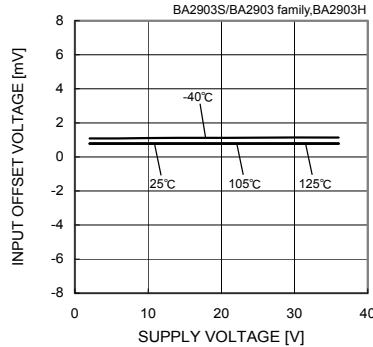
Fig. 48 Input Offset Voltage - Supply Voltage
