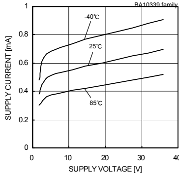
Fig. 22 Supply Current - Supply Voltage
