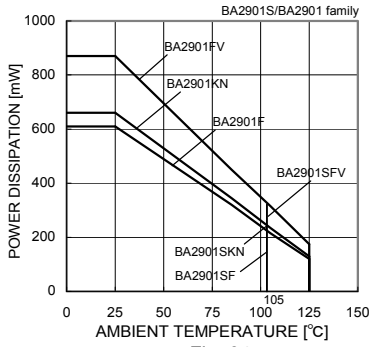
Fig. 64 Derating Curve
