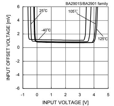
Fig. 81 Input Offset Voltage - Input Voltage (VCC=5V)
