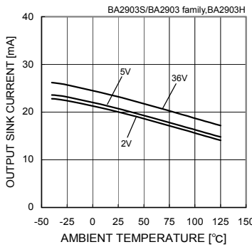
Fig. 47 Output Sink Current - Ambient Temperature (VOUT=1.5[V])
