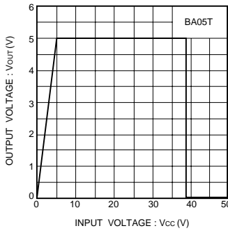
Fig. 10 Over voltage protection characteristics
