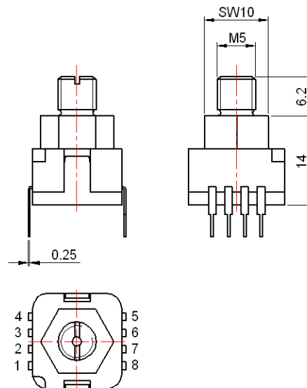
Type KC (M5 thread connection)
