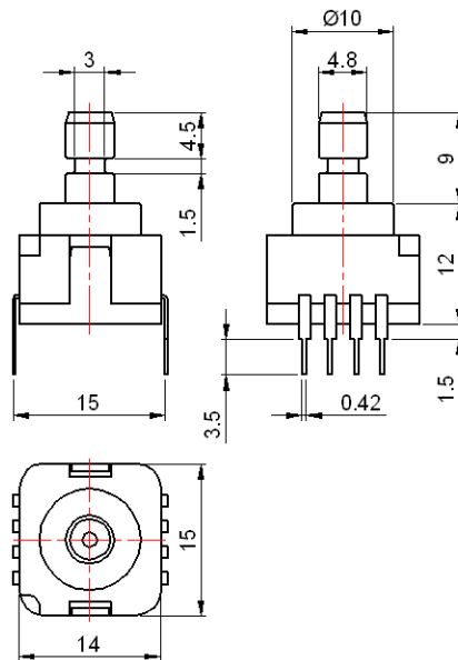
Type KD (4.8 mm tube fitting)
