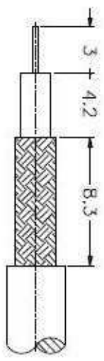
RECOMMENDED CABLE STRIPPING DIM'S
