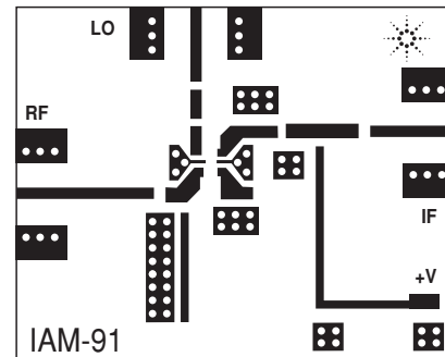
Figure 28. PCB Layout.
