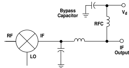
Figure 25. Bias Connection.
