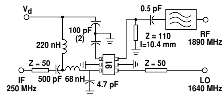
Figure 18. Test Circuit.
