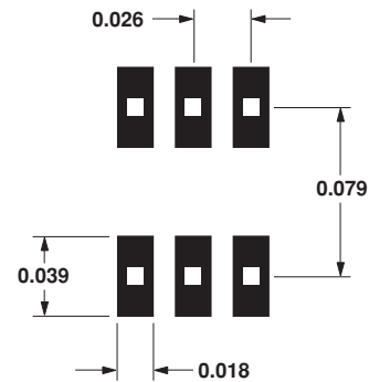
Figure 35. Recommended PCB Pad Layout for Avago's SC70 6L/SOT-363 Products.
