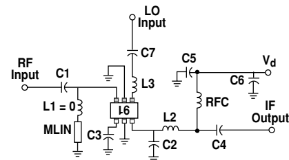
Figure 29. Schematic of Example Application Circuit.
