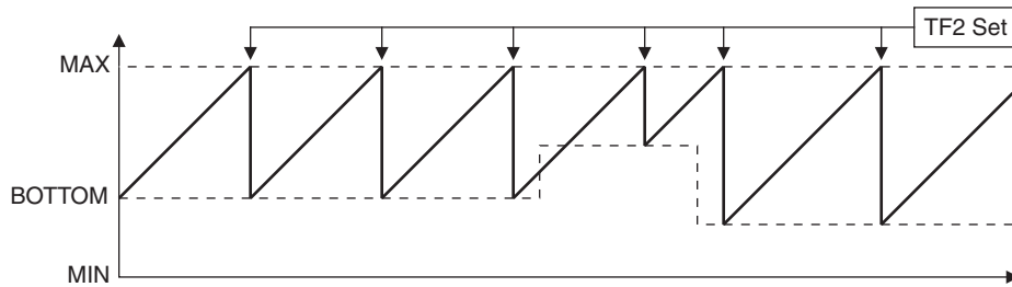
Figure 12-3. Timer 2 Waveform: Auto-Reload Mode (DCEN = 0)
