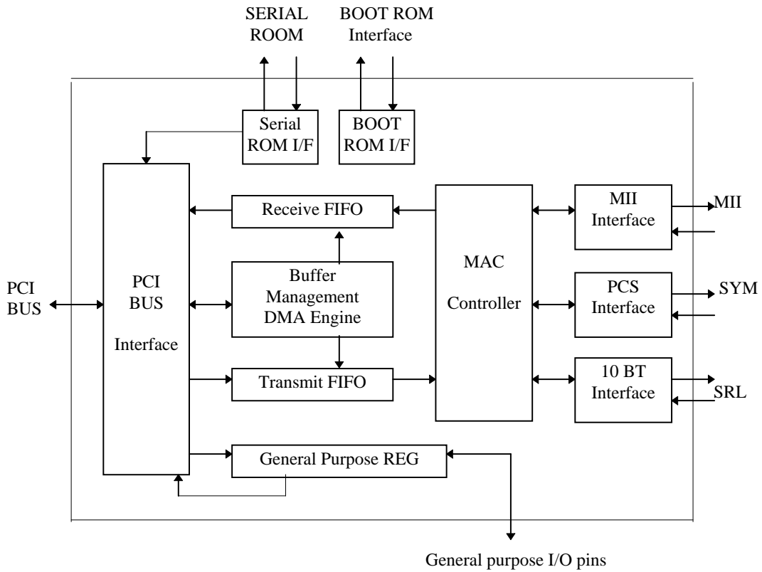
Fig - 1 AX88140A Block Diagram
