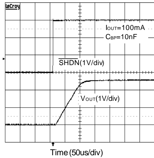
Exiting Shutdown Waveform
