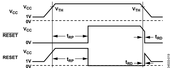
Figure 17. Reset Timing Diagram
