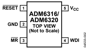
Figure 3. ADM6316/ADM6320 Pin Configuration
