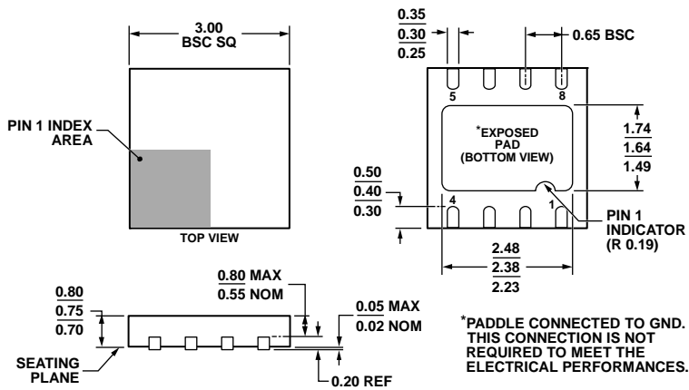
Figure 27. 8-Terminal Quad Flat No Lead Package (QFN) [LFCSP_WD] 3 mm x 3 mm Body, Very Very Thin, Dual Lead (CP-8-3)
