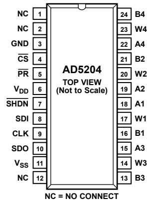
Figure 6. AD5204 SOIC/TSSOP/PDIP Pin Configuration
