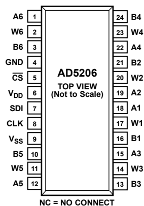
Figure 8. AD5206 SOIC/TSSOP/PDIP Pin Configuration
