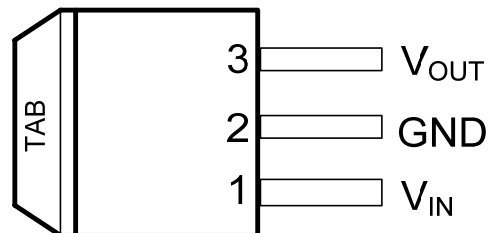
3-Pin TO-263 (M)
