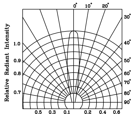
RADIATION DIAGRAM
