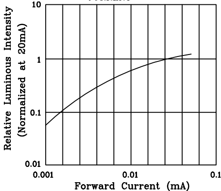
RELATIVE RADIANT INTENSITY VS. FORWARD CURRENT
