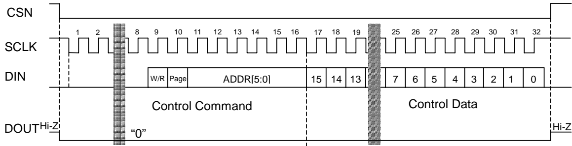
Figure 10. Write Operation
