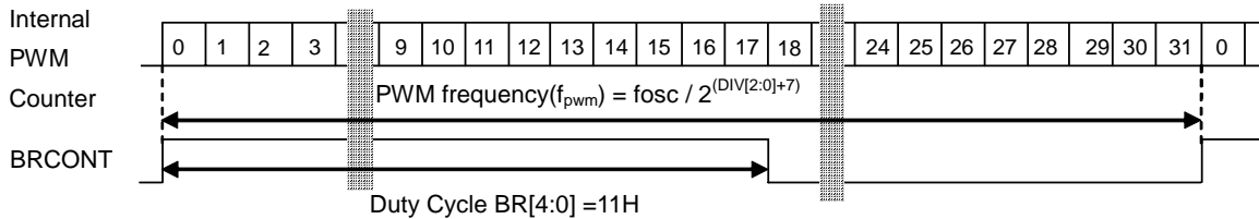
Figure 16. PWM output waveform
