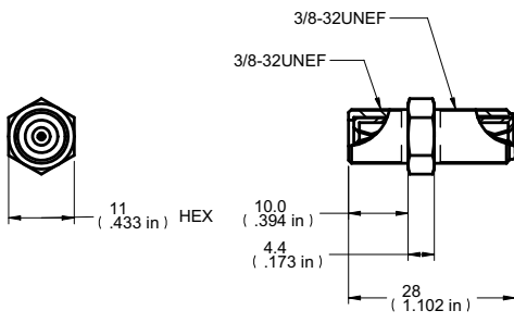
DIM OUTLINE
