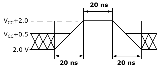
Figure 9. Maximum Positive Overshoot Waveform
