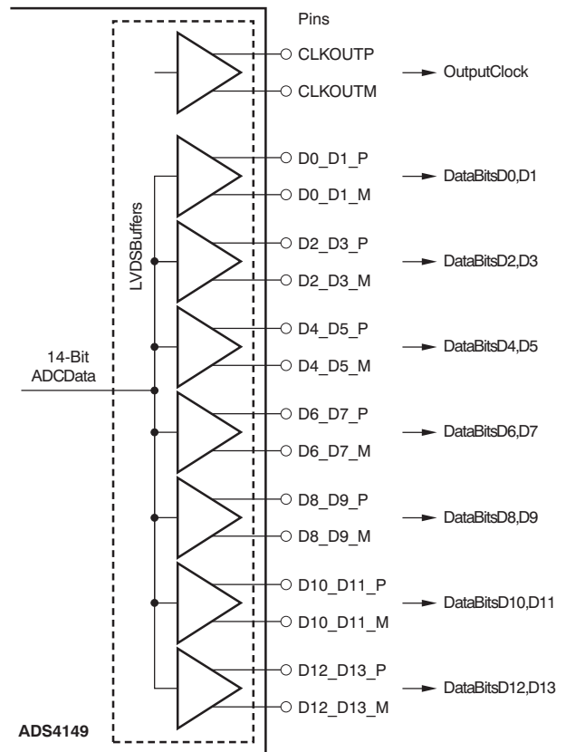
Figure 125. ADS414x LVDS Data Outputs
