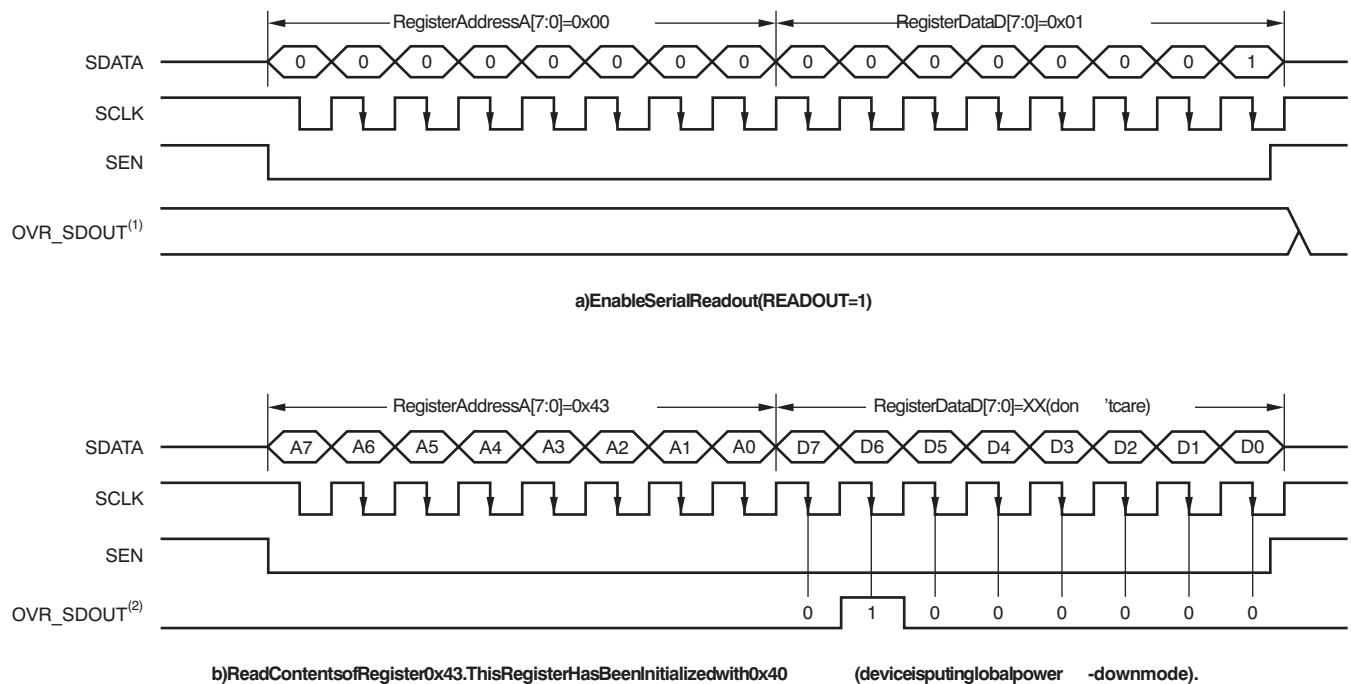
Figure 13. Serial Readout Timing Diagram
