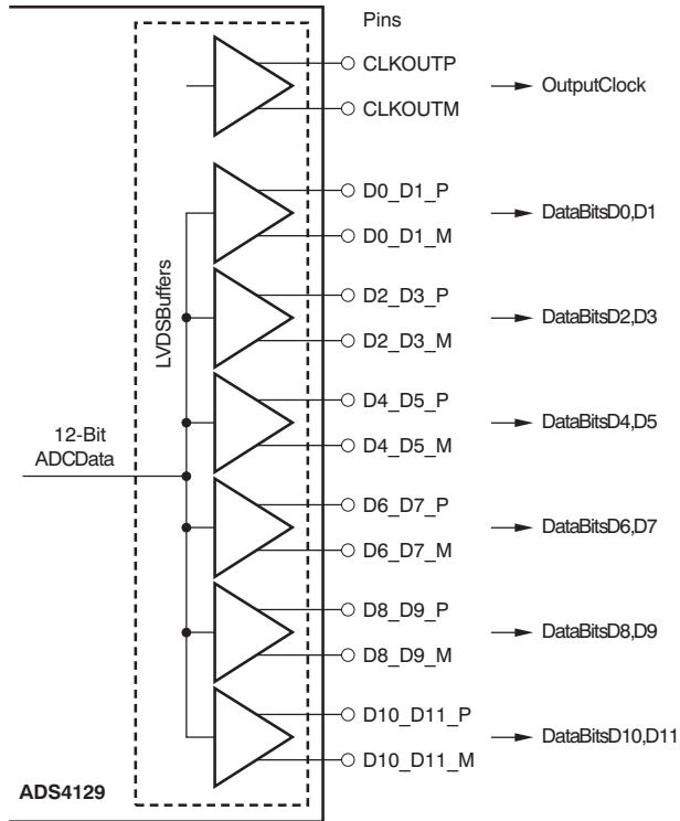
Figure 124. ADS412x LVDS Data Outputs
