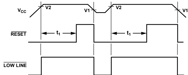
t_1 = RESET TIME V_1 = RESET VOLTAGE THRESHOLD LOW V_2 = RESET VOLTAGE THRESHOLD HIGH HYSTERESIS = V_2 - V_1
