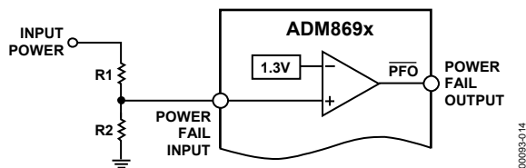
Figure 23. Power-Fail Comparator
