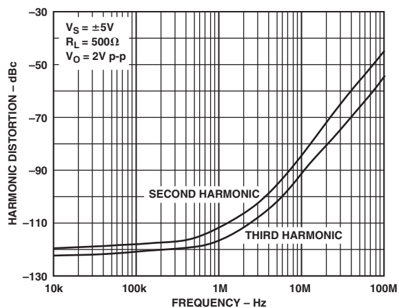
Figure 1. AD9631 Harmonic Distortion vs. Frequency, G = +1
