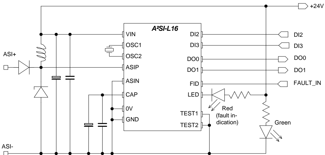
Figure 5-2: Typical application II
