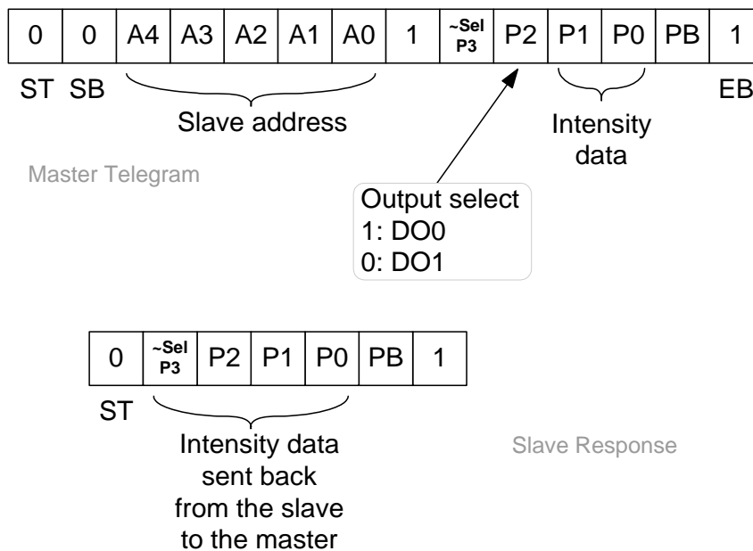
Figure 4-3: PWM control
