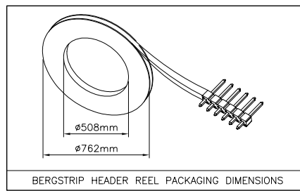
BERGSTRIK HEADER REEL PACKAGING DIMENSIONS
