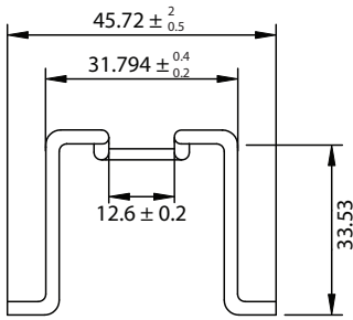
CLIP 1.80 ± 0.03mm Dia. Stainless Steel Wire
