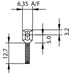
SCREW 6 BA Brass, Nickel Plated
