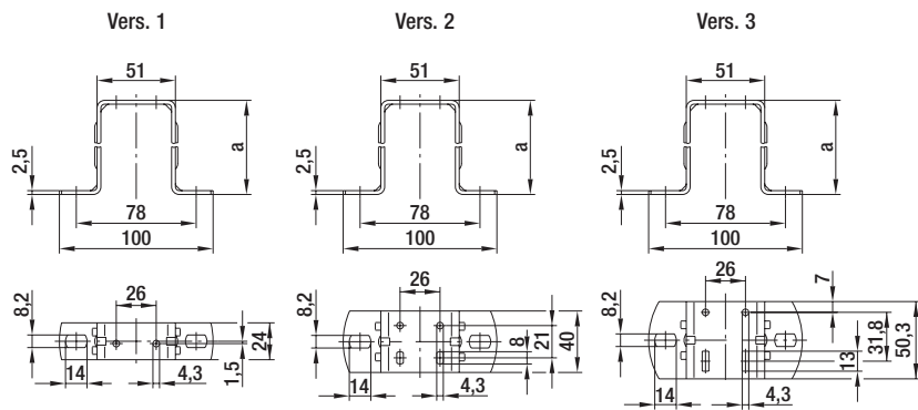
Mounting brackets for Q-motors (foot measure 26 mm)
