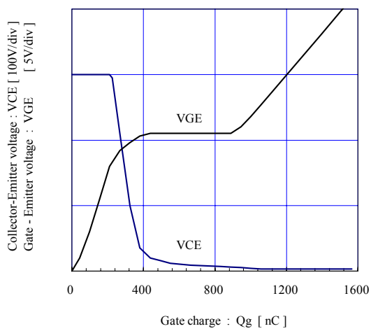
Dynamic Gate charge (typ.)
