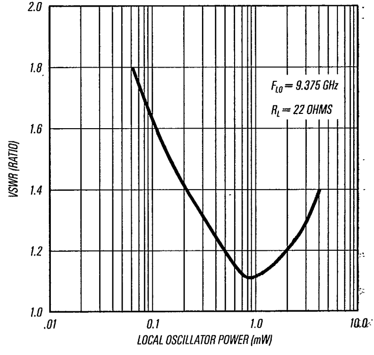
VSWR VS LOCAL OSCILLATOR POWER
