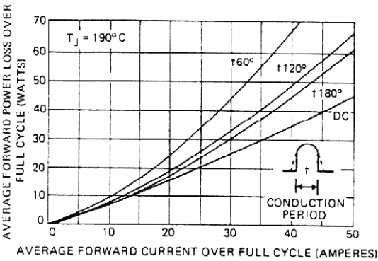
Fig. 2 - Typical Low Level Forward Power Loss vs. Average Forward Current (Sinusoidal Current Waveform), 1N1183 and 1N3765 Series
