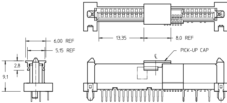
PART WITH PICK-UP CAP, SEE NOTE ⑤
