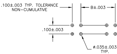
RECOMMENDED HOLE LAYOUT
